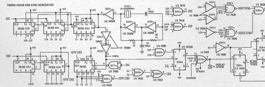
FIG. 1—COMPLETE SCHEMATIC OF 2650-based microcomputer. All circuitry, including cassette-tape interface and video display generator, mount on single PC-board. Connection to peripheral devices is made via six IC sockets.
